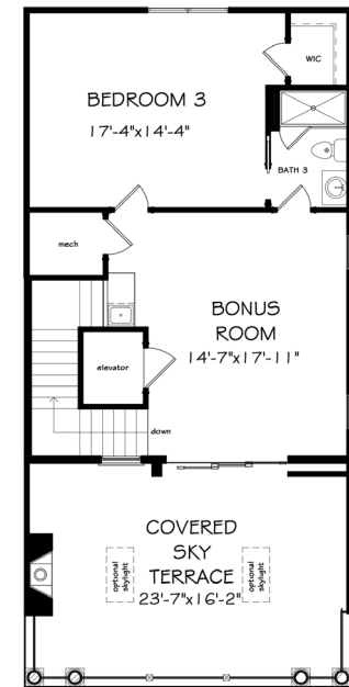
THIRD FLOOR
