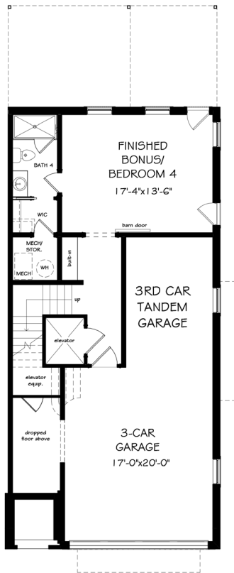
TERRACE LEVEL
