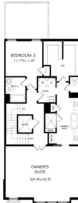
SECOND FLOOR
