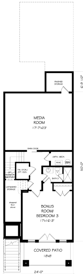
TERRACE LEVEL
