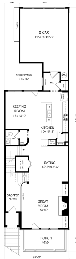
FIRST FLOOR
