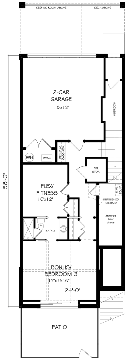
TERRACE LEVEL
