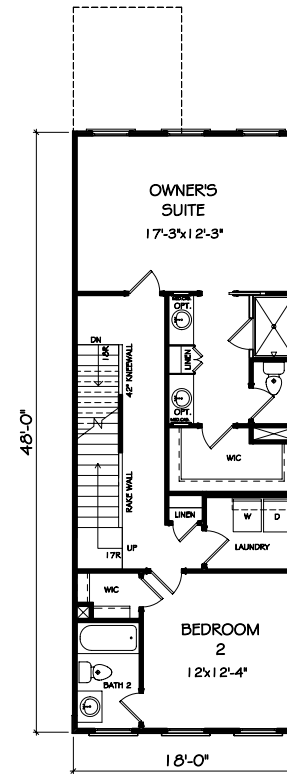
SECOND FLOOR
