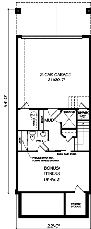
TERRACE LEVEL
