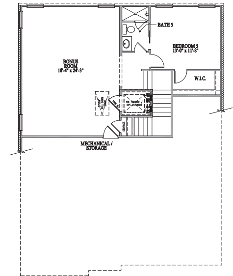
THIRD FLOOR
