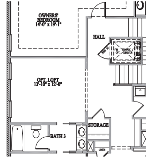
OPTIONAL SECOND FLOOR LOFT
